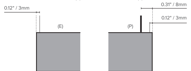
SUSPENSION POINT LOCATIONS POWERED (P) AND UNPOWERED END (E)
